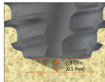
Minimized tip extension of the drill
