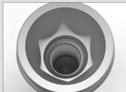
Internal hex 11° taper connection
