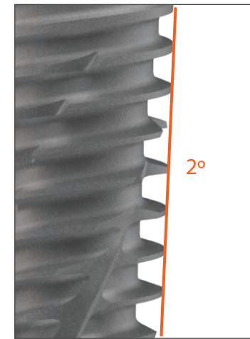
2° taper body - Advantageous for immediate & early loading on soft bone
